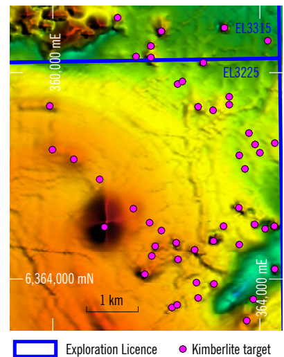
Figure 3 Detailed image showing kimberlite pipe targets from the south east corner of the new Nackara 2 helimag survey.
