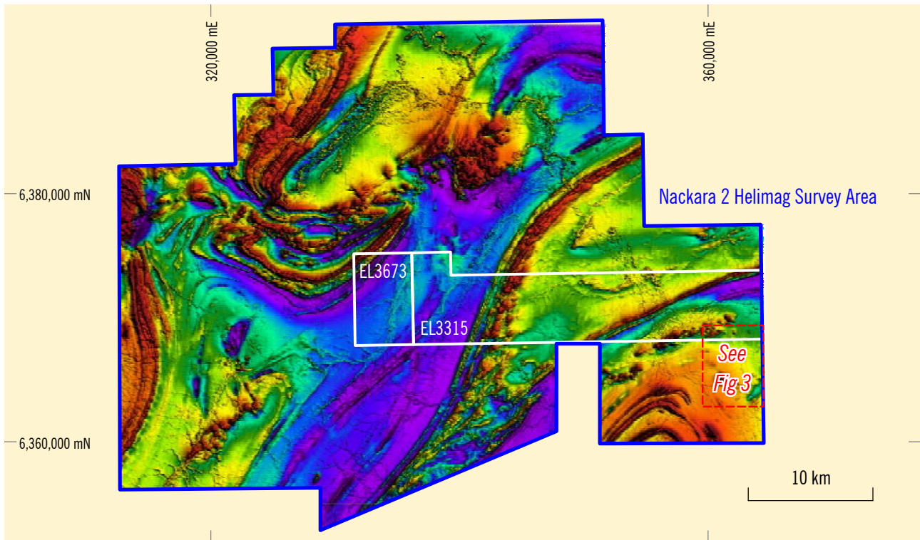
Figure 2 Total Magnetic Intensity image from the recently-completed Nackara 2 Helimag survey. Red areas are highly magnetic and blue-purple areas have low magnetic intensities. ELs 3315 and 3673 form the new joint venture with Primary Resources Limited.
