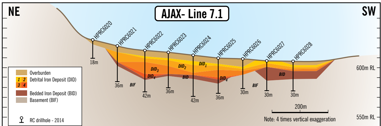
Figure 4 Line 7.1 cross-section through the Ajax deposit.
