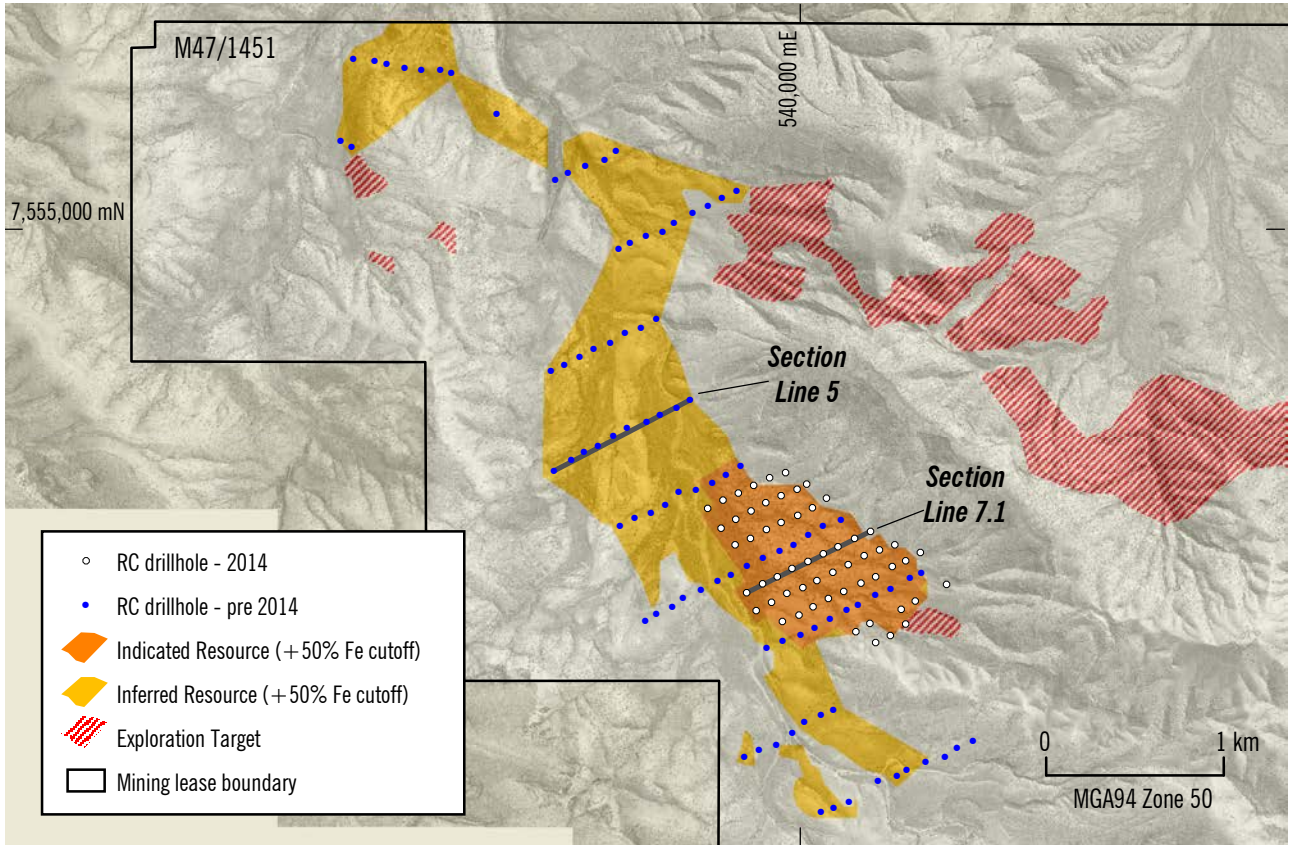
Figure 2 Ajax deposit drill hole plan.
