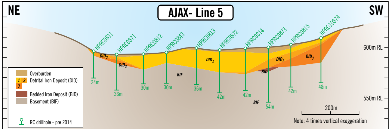
Figure 3 Line 5 cross-section through the Ajax deposit.
